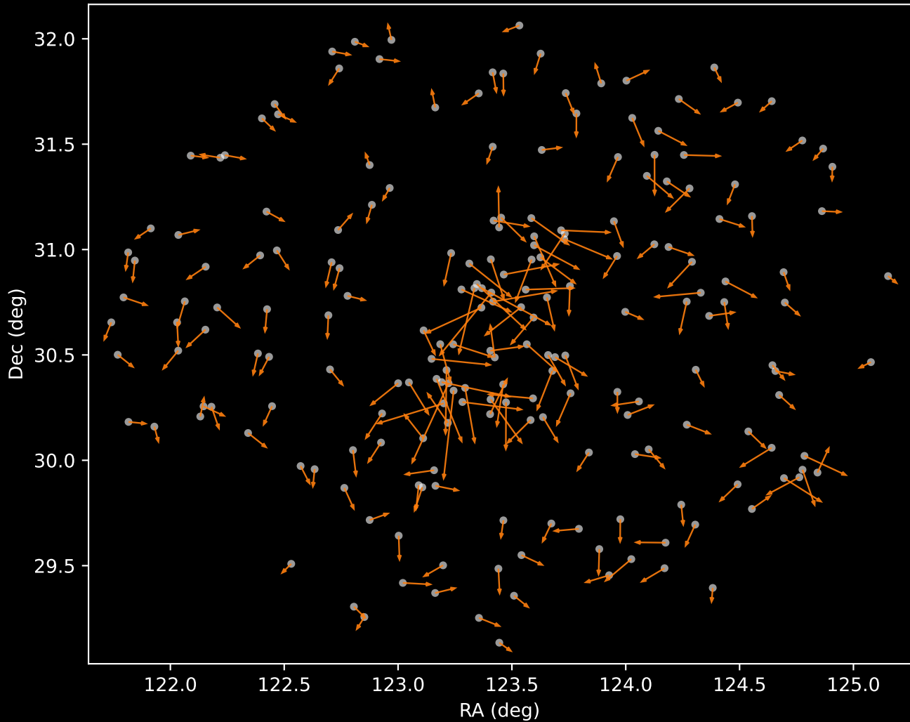
APOGEE DR17 Cluster 2 Proper Motion Vectors (n=205)
