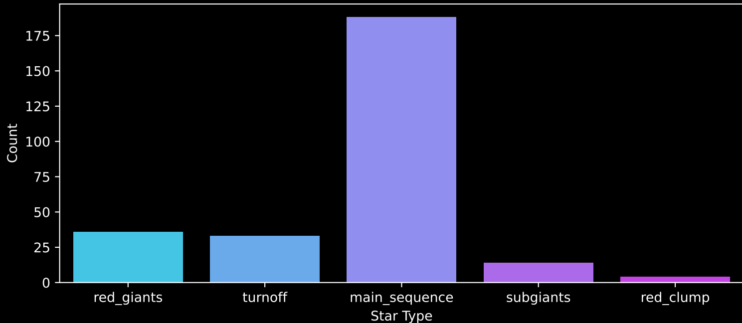
APOGEE DR17 Field: [M33] Count plot of Star Type
