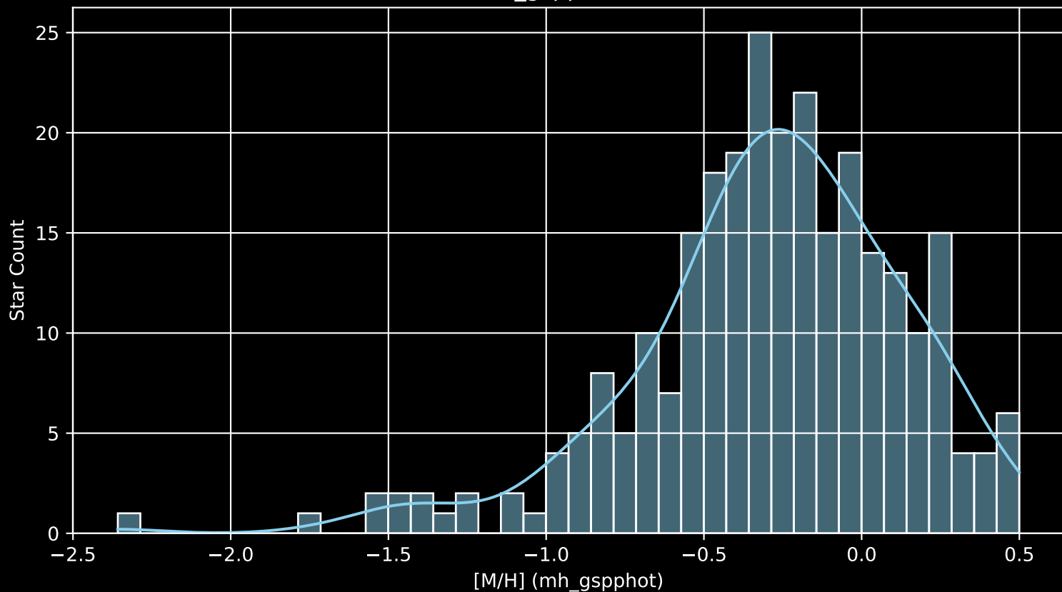
APOGEE DR17 Field: [M33 [M/H] (mh_gspphot) (n= 272)
