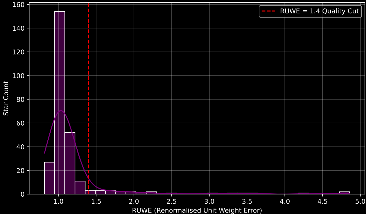
GAPOGEE DR17 Field [M33] RUWE Distribution (n= 268)
