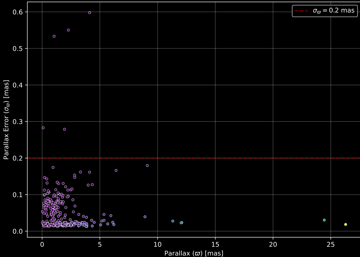
APOGEE DR17 Field: [M33] Parallax Quality (n= 275)
