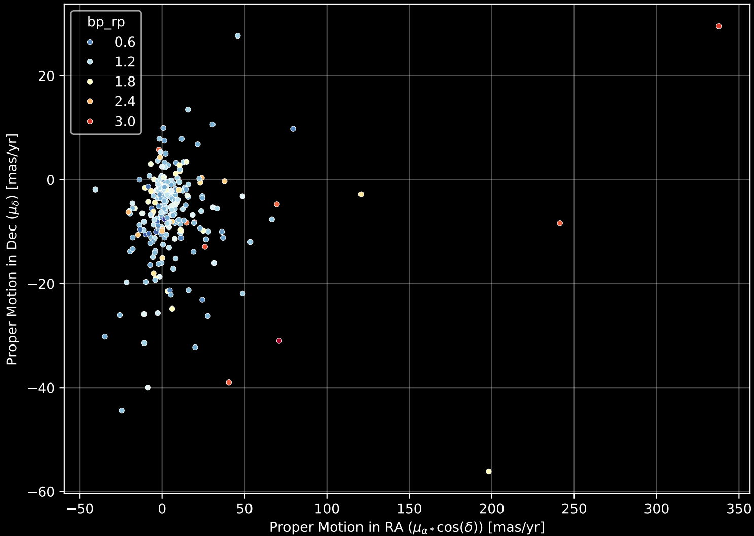
APOGEE DR17 Field: [M33] Proper Motion Diagram (n= 275)
